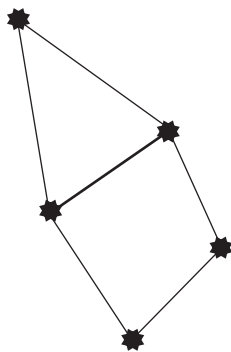
Cepheus (5 stars):
